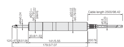
DK25NR5/PR5
