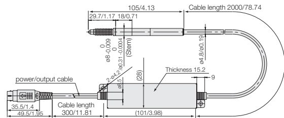
DK812AR/DK812AR5/DK812BR/DK812BR5
