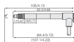
DK812AVR/DK812AVR5 DK812BVR5/DK812BVR5
