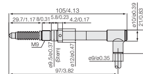
DK812AFLR/DK812AFLR5 DK812ABLR/DK812BFLR5
