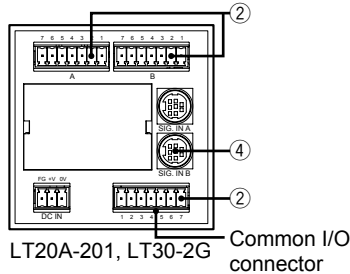
2 channel-models
