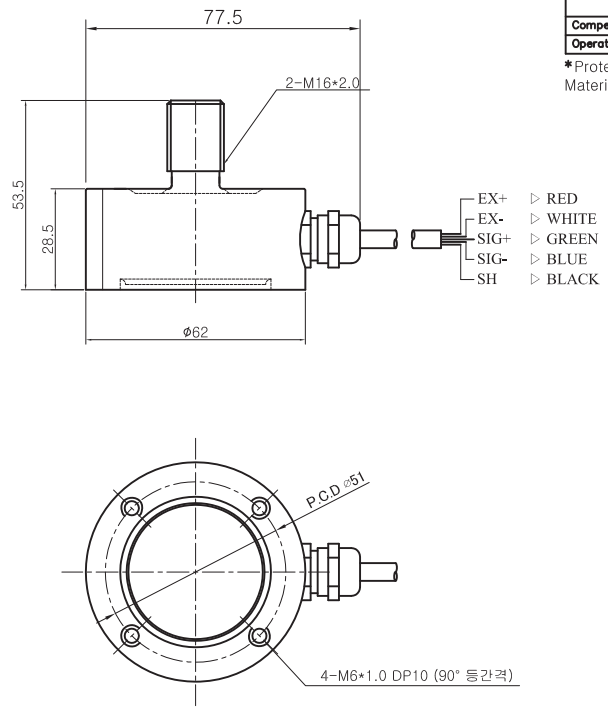
< ZMNT-1~2T Dimension >
