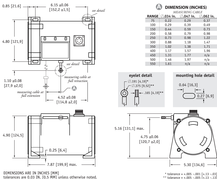
Fig. 1 – Outline Drawing
