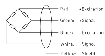
Cable Colour Code: (4-wire circuit)
